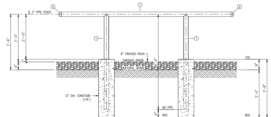
TYPICAL PIPE FENCE ELEVATION
