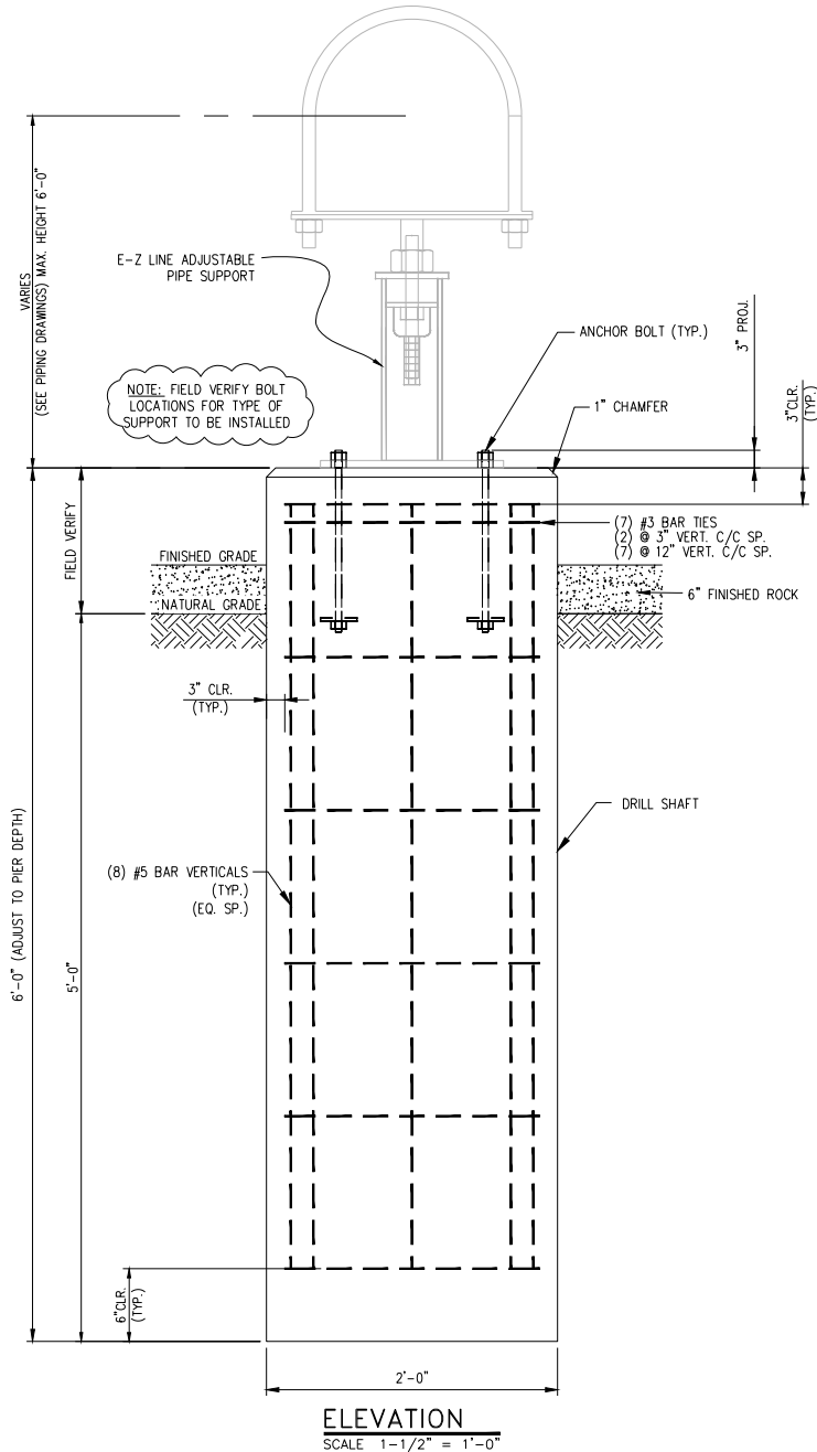
PIER SUPPORT DETAIL FOR EZ LINE SUPPORT 12" THRU 24" (1 REQUIRED)
