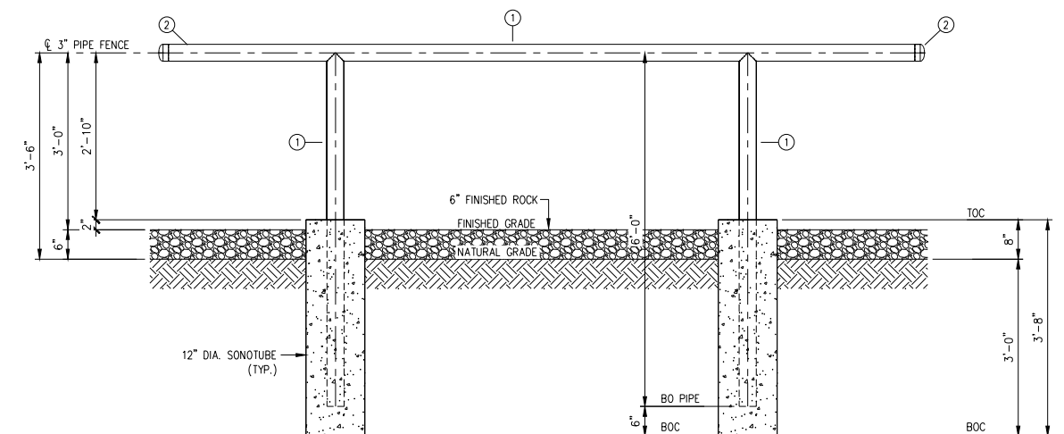
TYPICAL PIPE FENCE ELEVATION
