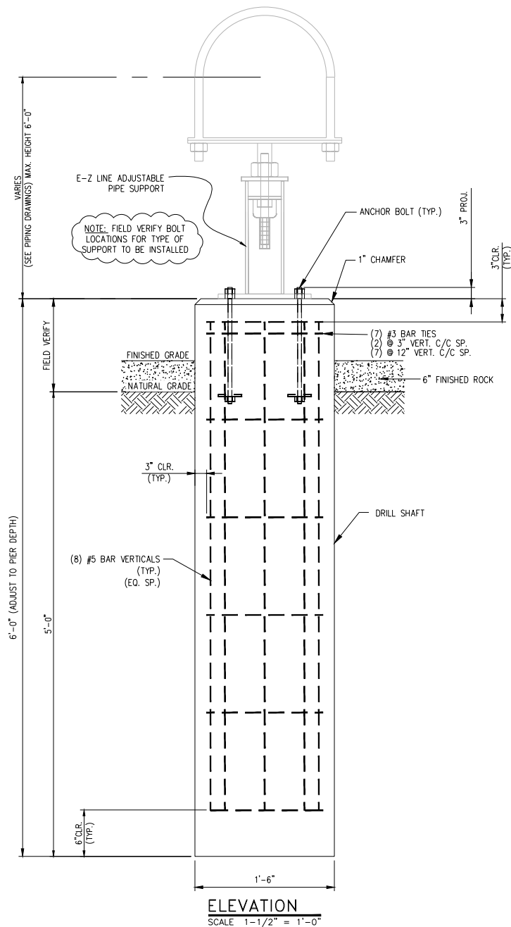
PIER SUPPORT DETAIL FOR E-Z LINE SUPPORT 2" THRU 10" (18 REQUIRED)
