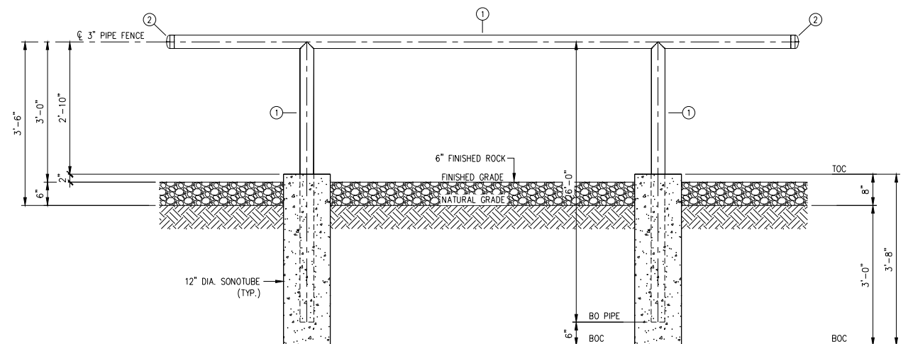
TYPICAL PIPE FENCE ELEVATION
